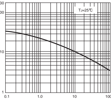
FIG. 5-TYPICAL JUNCTION CAPACITANCE
